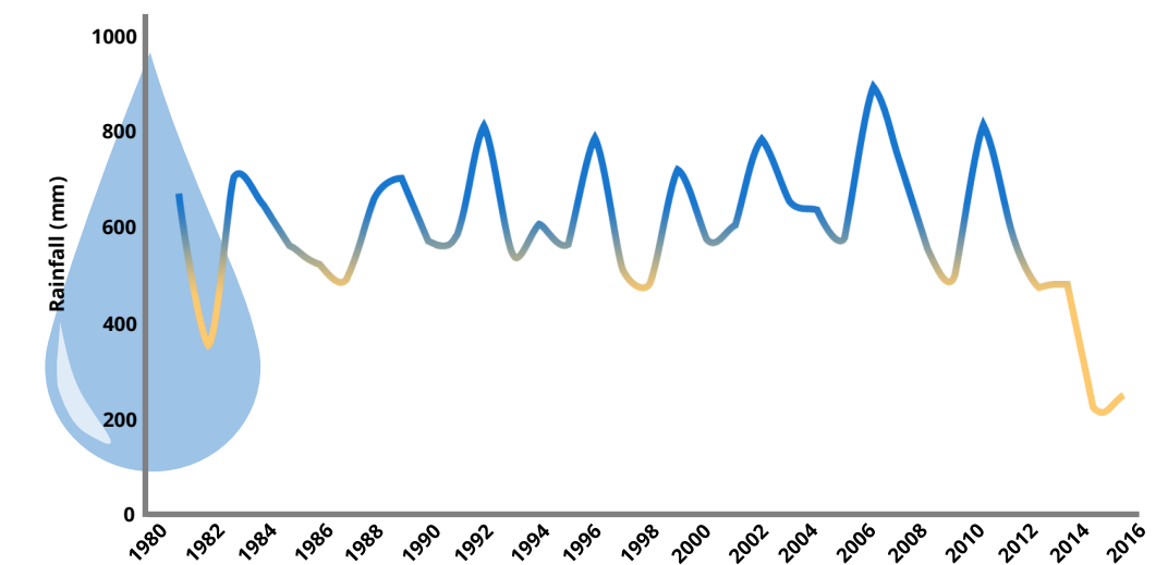
Figure 3.8 Rainfall pattern of Mandalay in the Dry Zone of Myanmar, 1981-2016.
