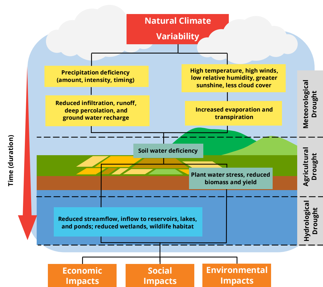
Figure 5.2 Cascading sequence of drought types and their impacts. All droughts begin as meteorological (source: Wilhite, 2000).
