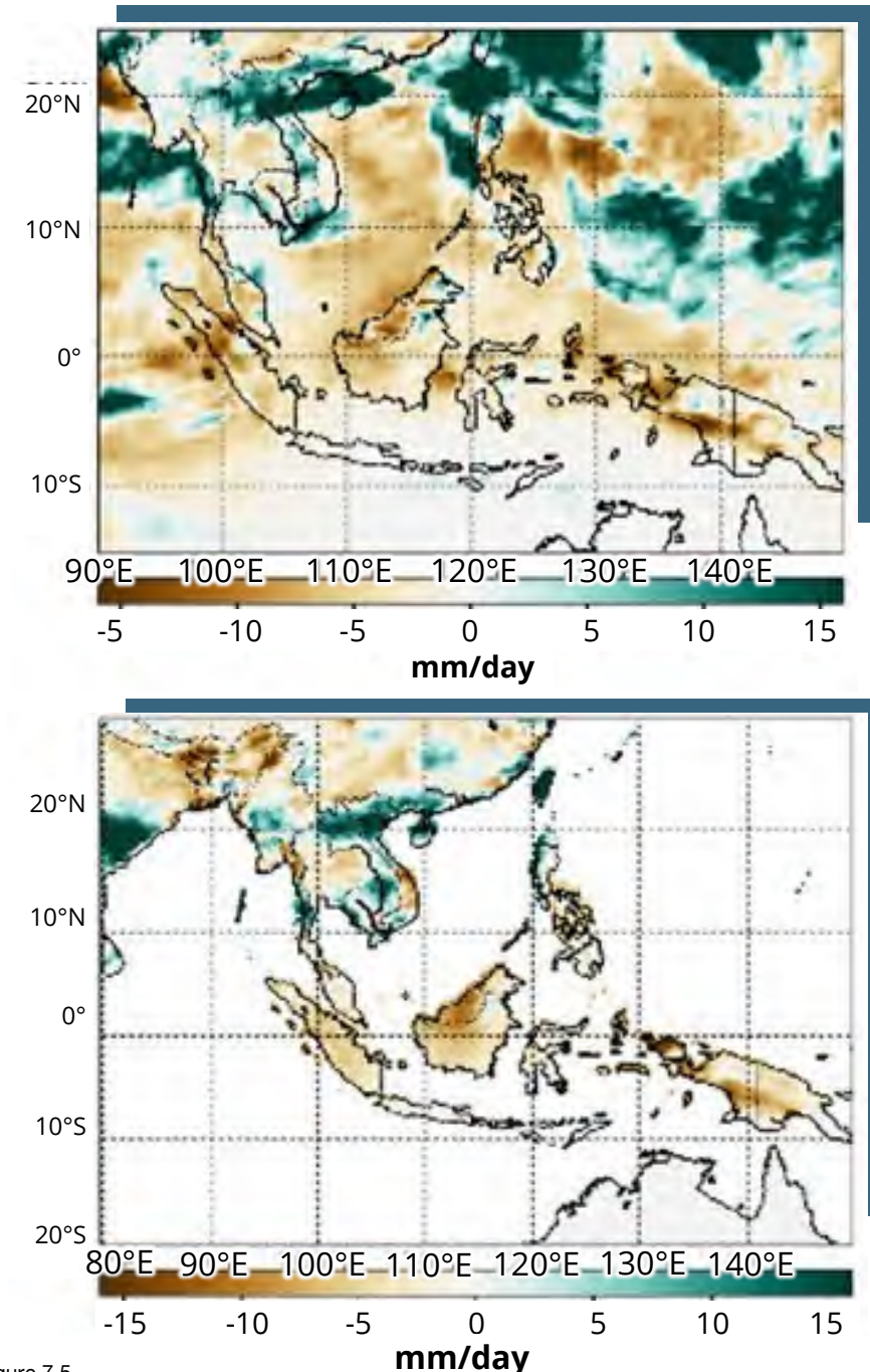
Figure 7.5 Rainfall anomaly (departure from the climatological mean) plot from two different datasets: CMORPH (top) and CHIRPS (bottom). Data are for Southeast Asia from 13 to 19 August 2018 with reference to the same week's climatology from 1998 to 2016 for CMORPH and 1997–2016 for CHIRPS. Negative anomaly (drier) conditions appear as shades of brown.
