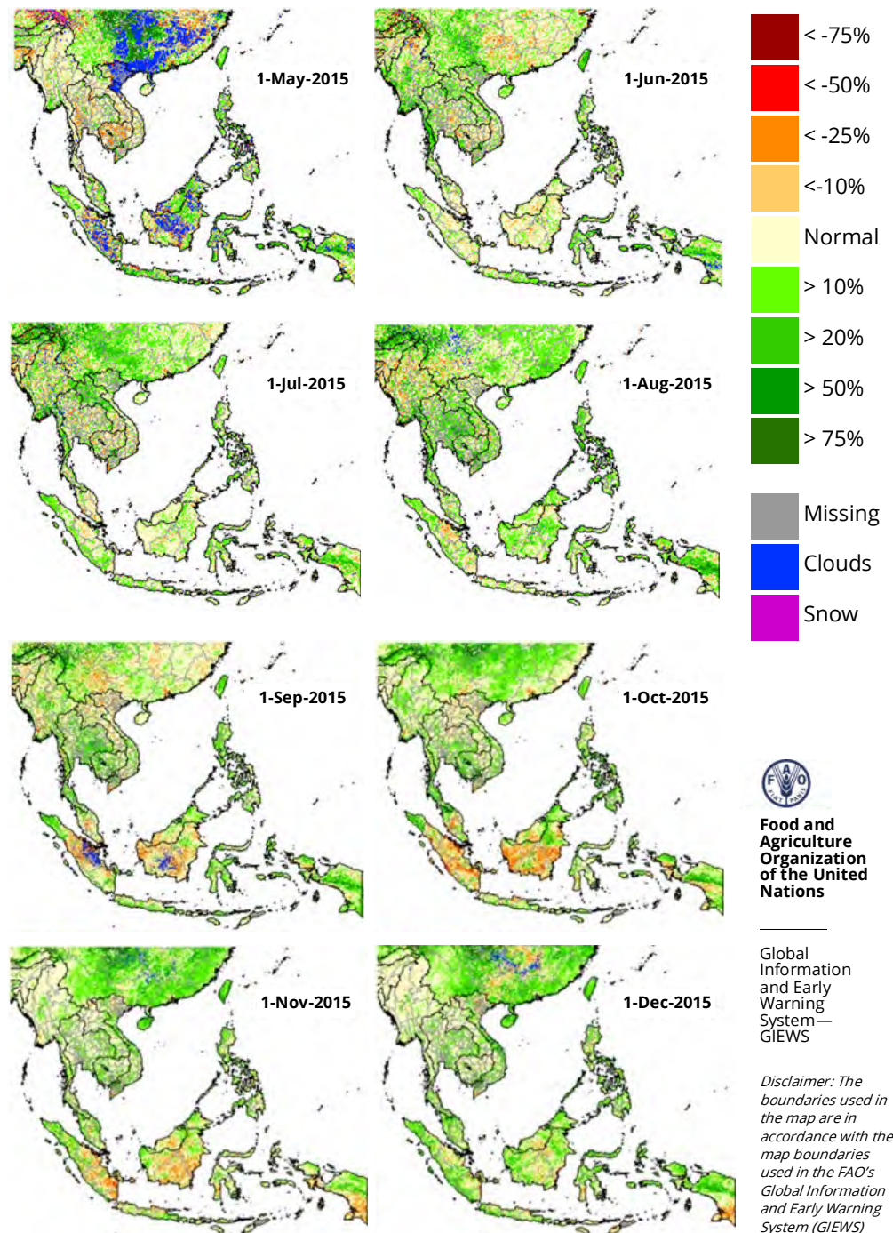
Figure 3.7 (a) Maps showing the NDVI anomaly from May to December 2015
