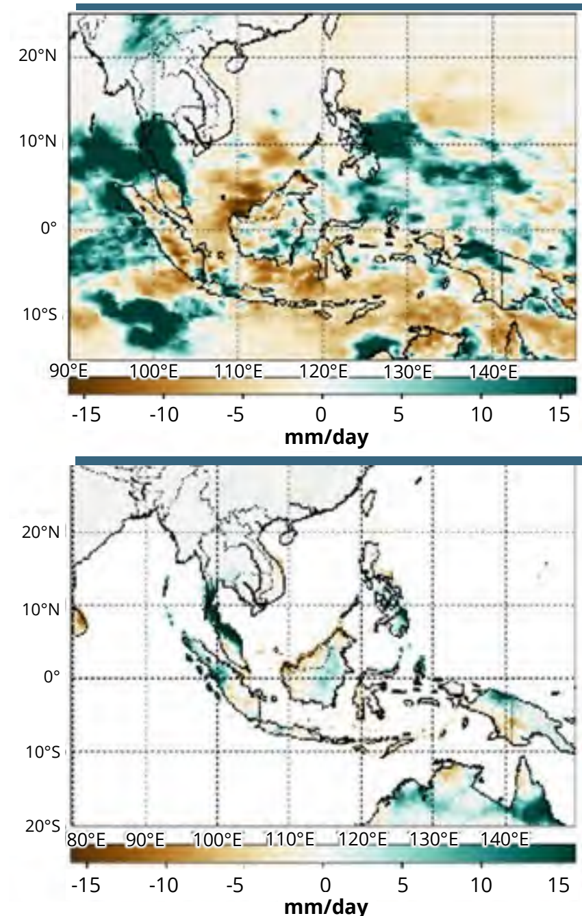
Figure 7.2 Rainfall anomaly (departure from the climatological mean) plot from two different datasets: CMORPH (top) and CHIRPS (bottom). Data are for Southeast Asia from 2 to 8 January 2017 with reference to the same week's climatology from 1998 to 2016 for CMORPH and 1997–2016 for CHIRPS. Positive anomaly (wetter) conditions appear as shades of green.
